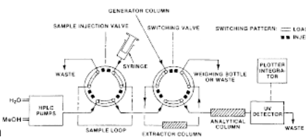
Figure 3—Schematic of HPLC—Generator Column Flow System
