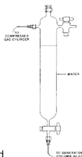
Figure 4—Water Reservoir for GC Method
