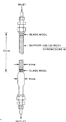
Figure 1—Generator Column
