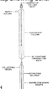
Figure 2—Setup Showing Generator Column Enclosed in a Water Jacket and Overall Arrangement of the Apparatus Used
